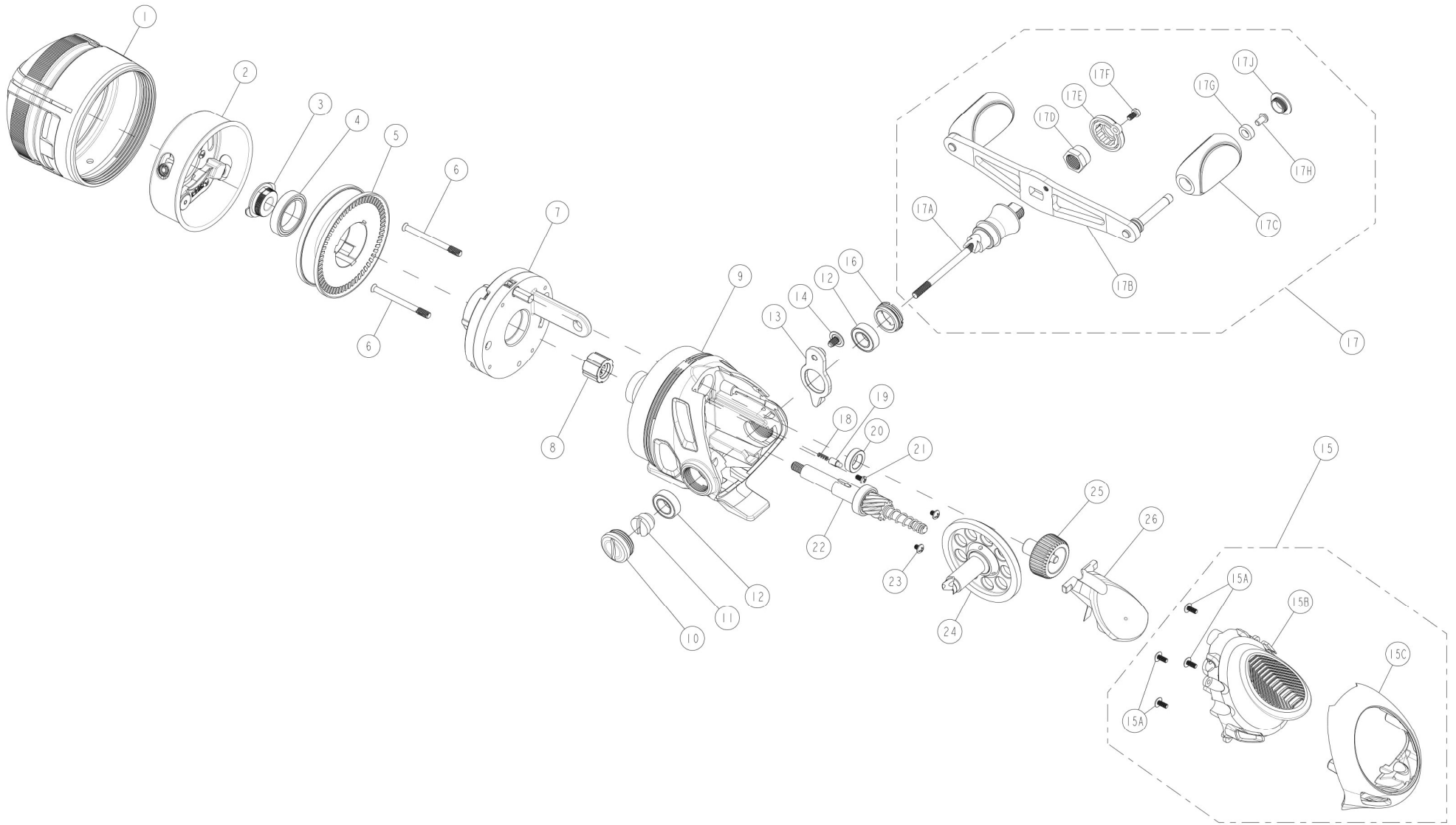
BULLET MG SPINCAST
